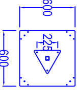
TRIANGLE SUPPORT + PEDESTAL
